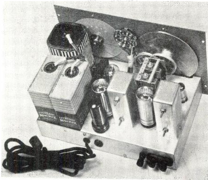
Careful planning permits a neat arrangement of parts plus battery space.
