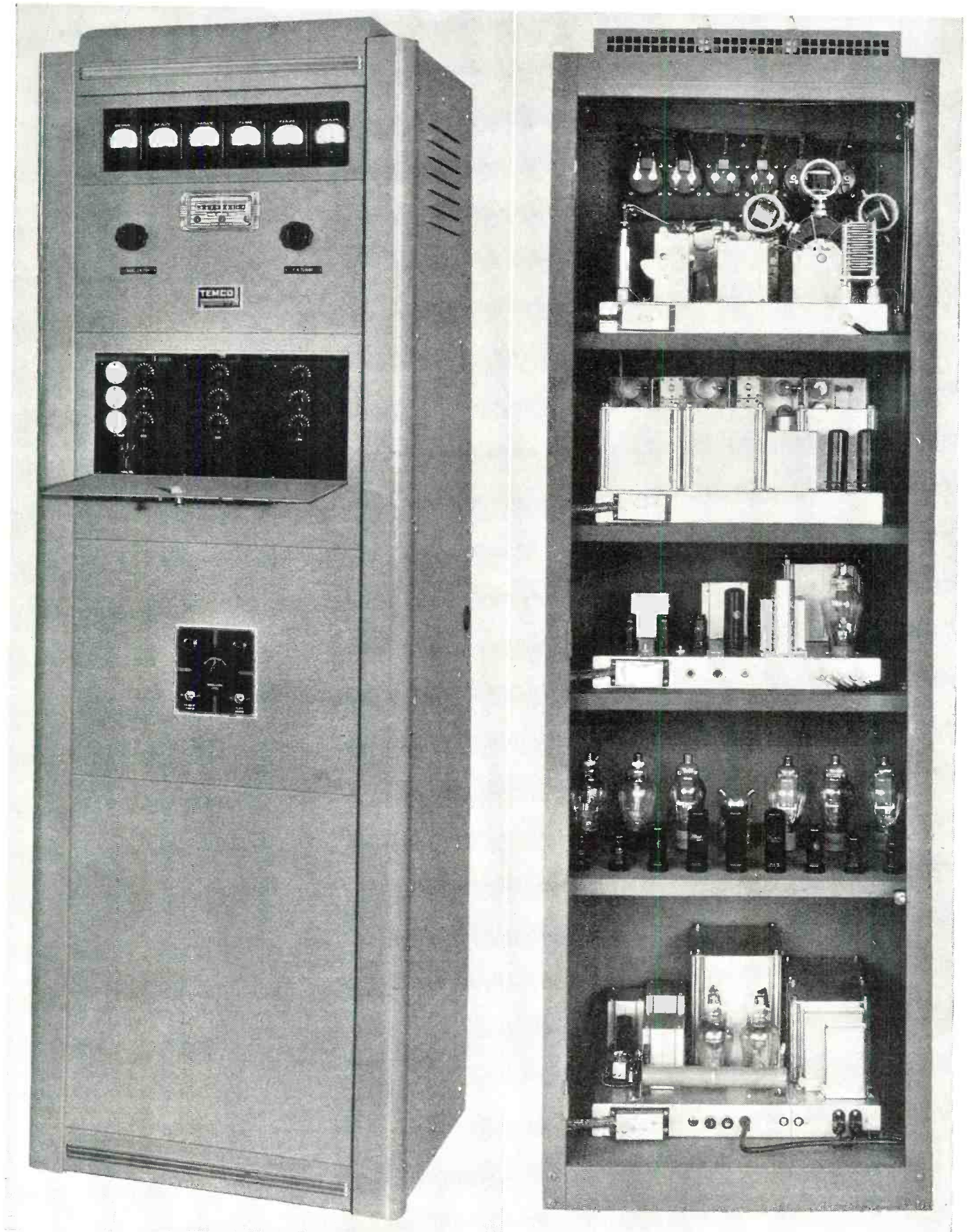
The TEMCO Model 250-G, 250 watt, three band radiotelephone and telegraph transmitter.
