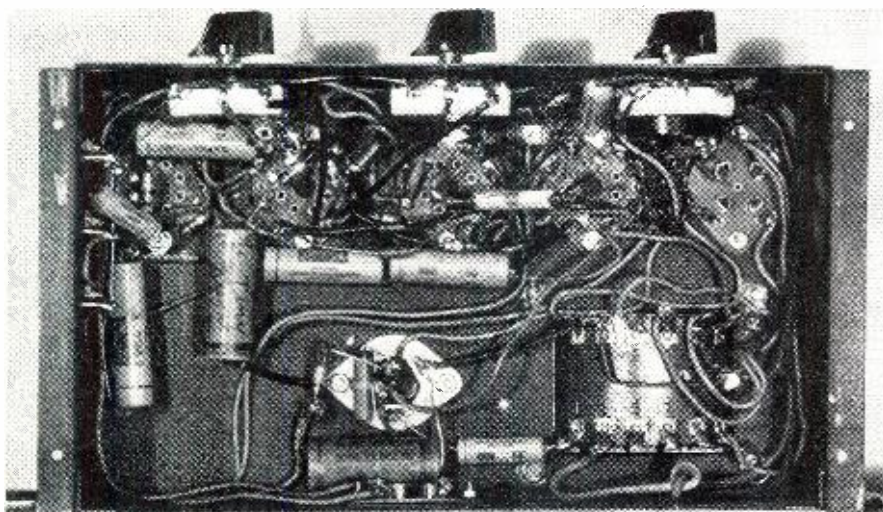
Underchassis view shows tube sockets lined up near front of chassis. The plate-and-filament transformer is farthest from the pre-amplifier stage.
