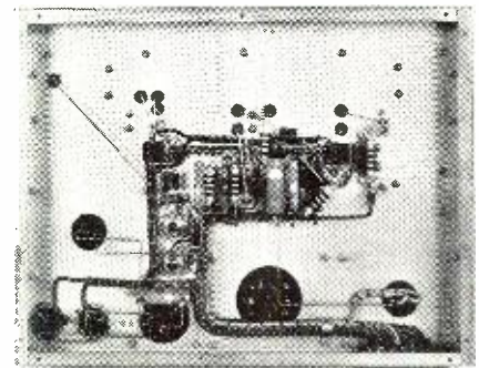
Above: Push-pull 812's used in the amplifier stage. Below: Under side of three-band exciter chassis.
