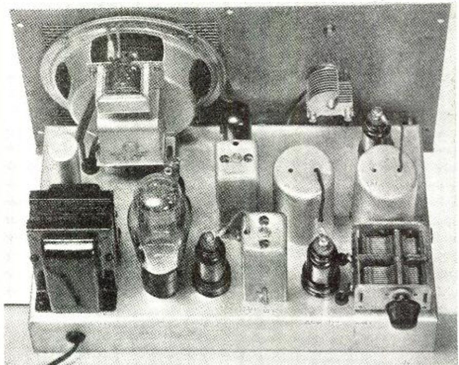
Standard parts are used for construction of the Channel Substitute. The antenna and r.f. condenser is shown mounted at the rear corner.
