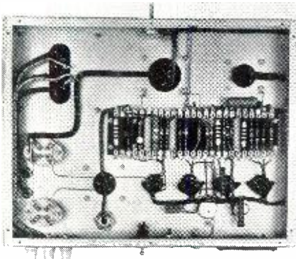
Underside of the speech amplifier.
