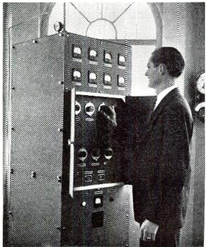
UHF traffic-control transmitter at Floyd Bennett airport. Tuning controls are placed behind metal doors. Note gas pressure gauge, on top, for co-axial feeder.
