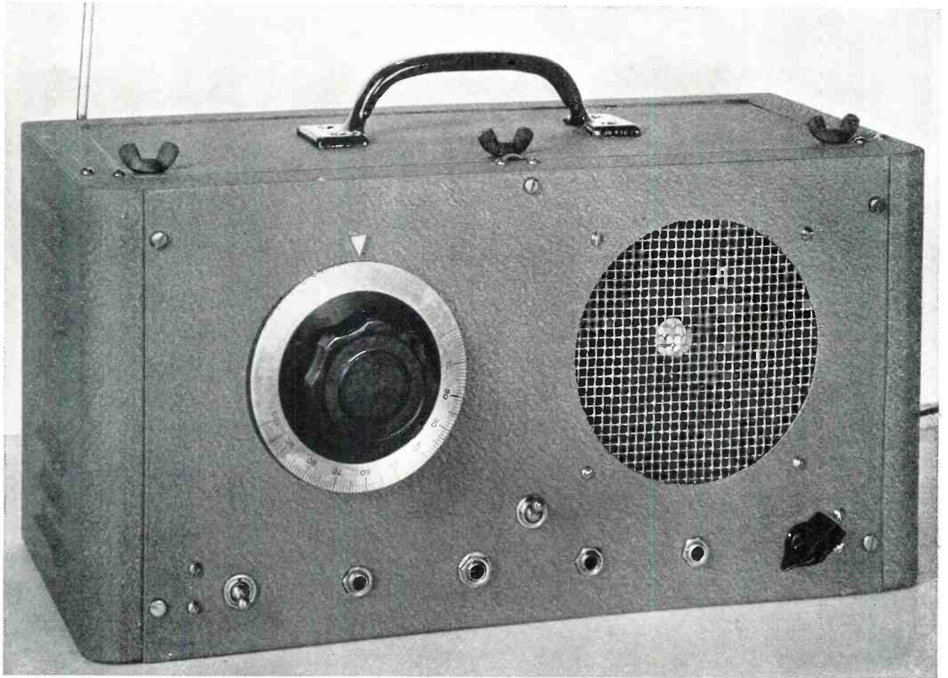
The finished Channel Substitute takes on the appearance of a commercially-built test instrument.
